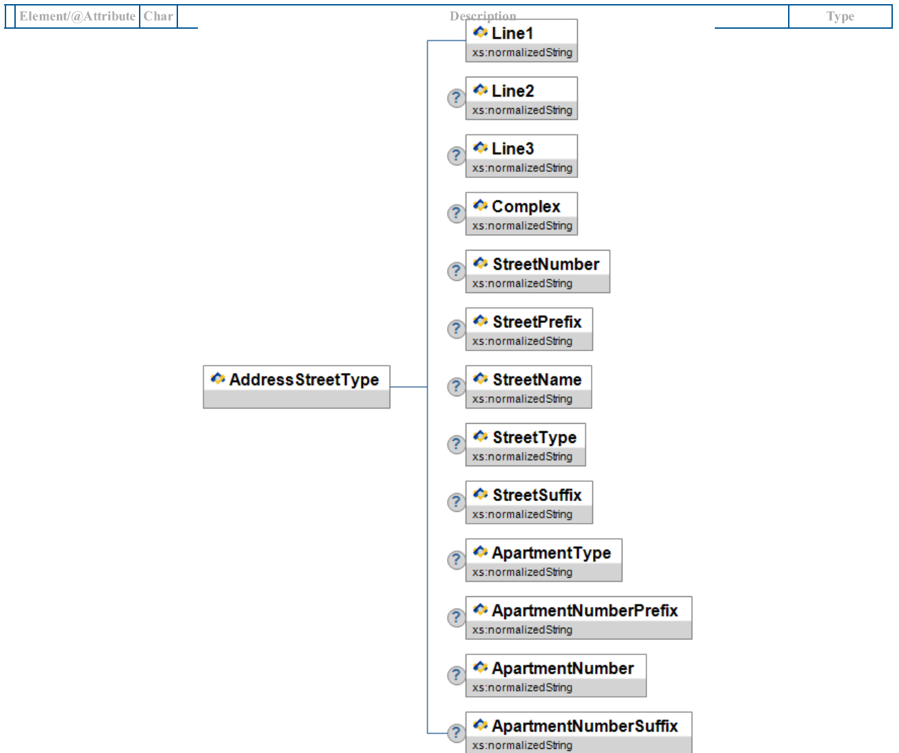
Figure A.7-1: AddressStreetType
