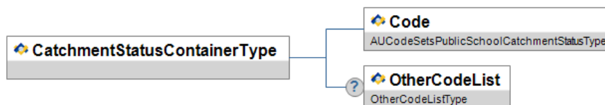
Figure A.29-1: CatchmentStatusContainerType
