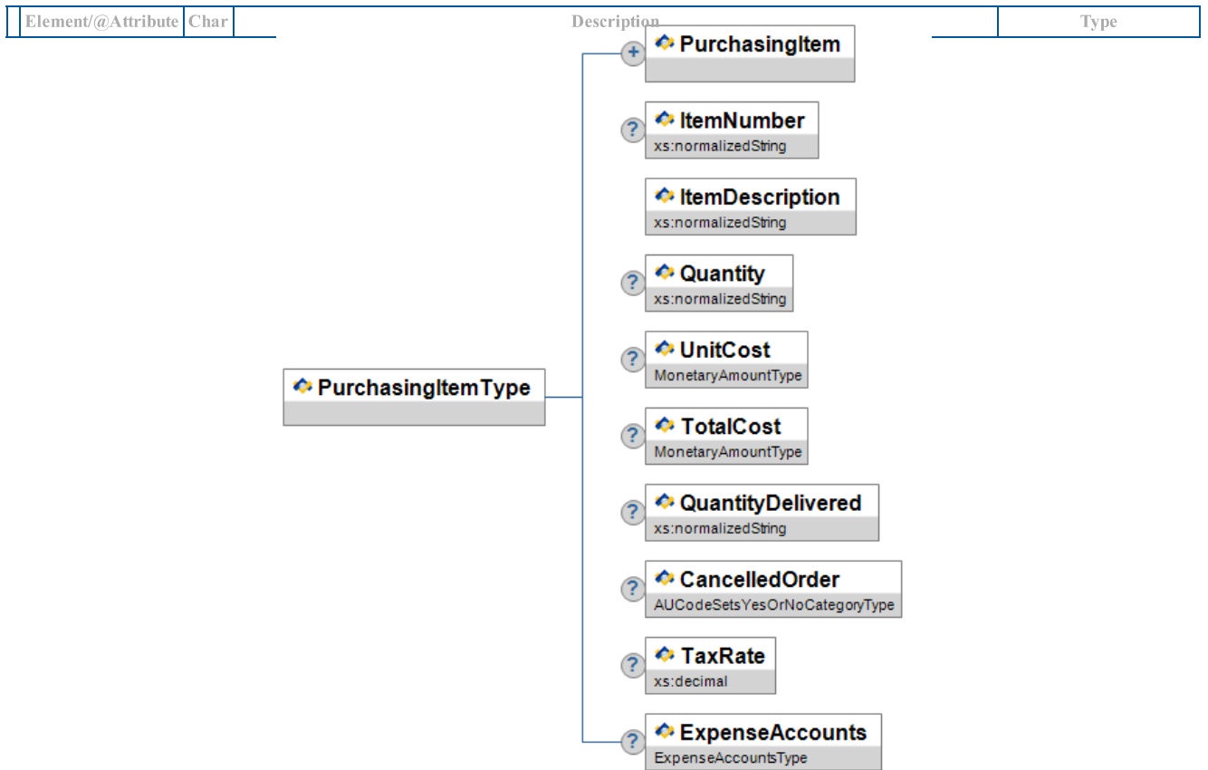
Figure A.121-1: PurchasingItemType
