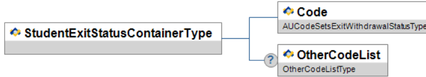
Figure A.167-1: StudentExitStatusContainerType
