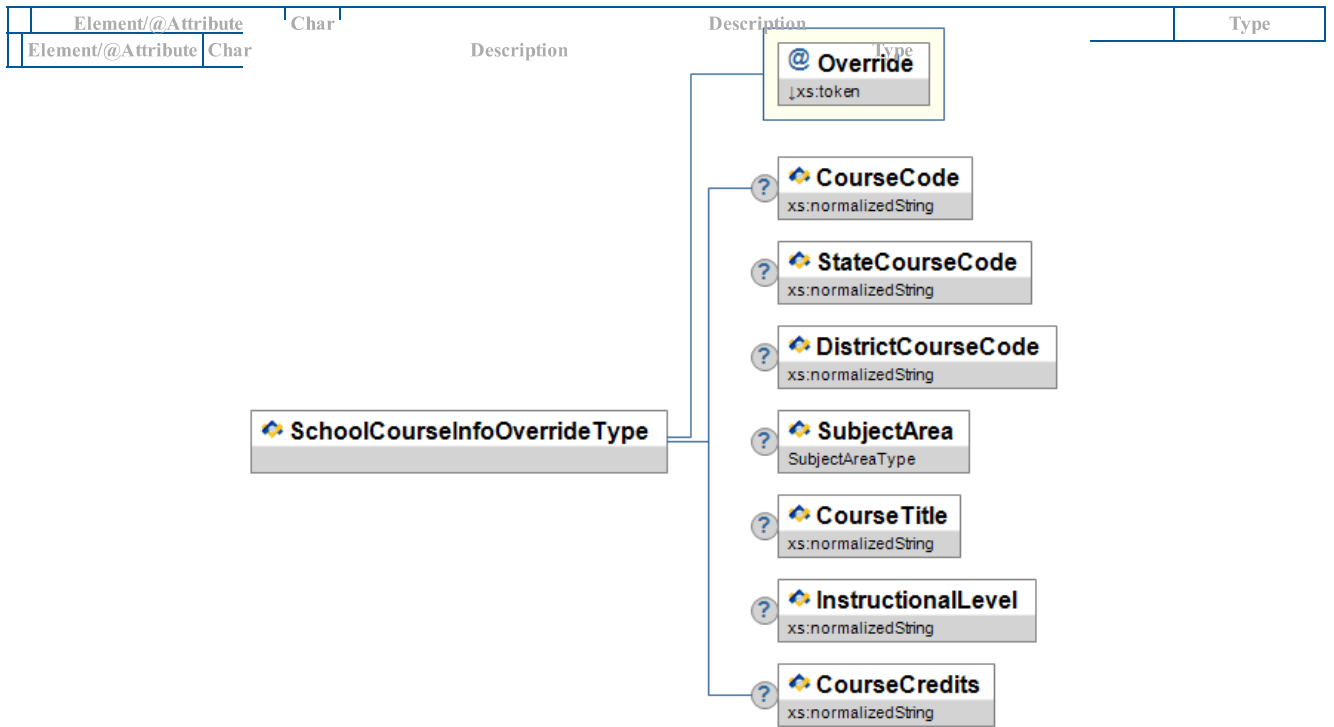
Figure A.137-1: SchoolCourseInfoOverrideType
