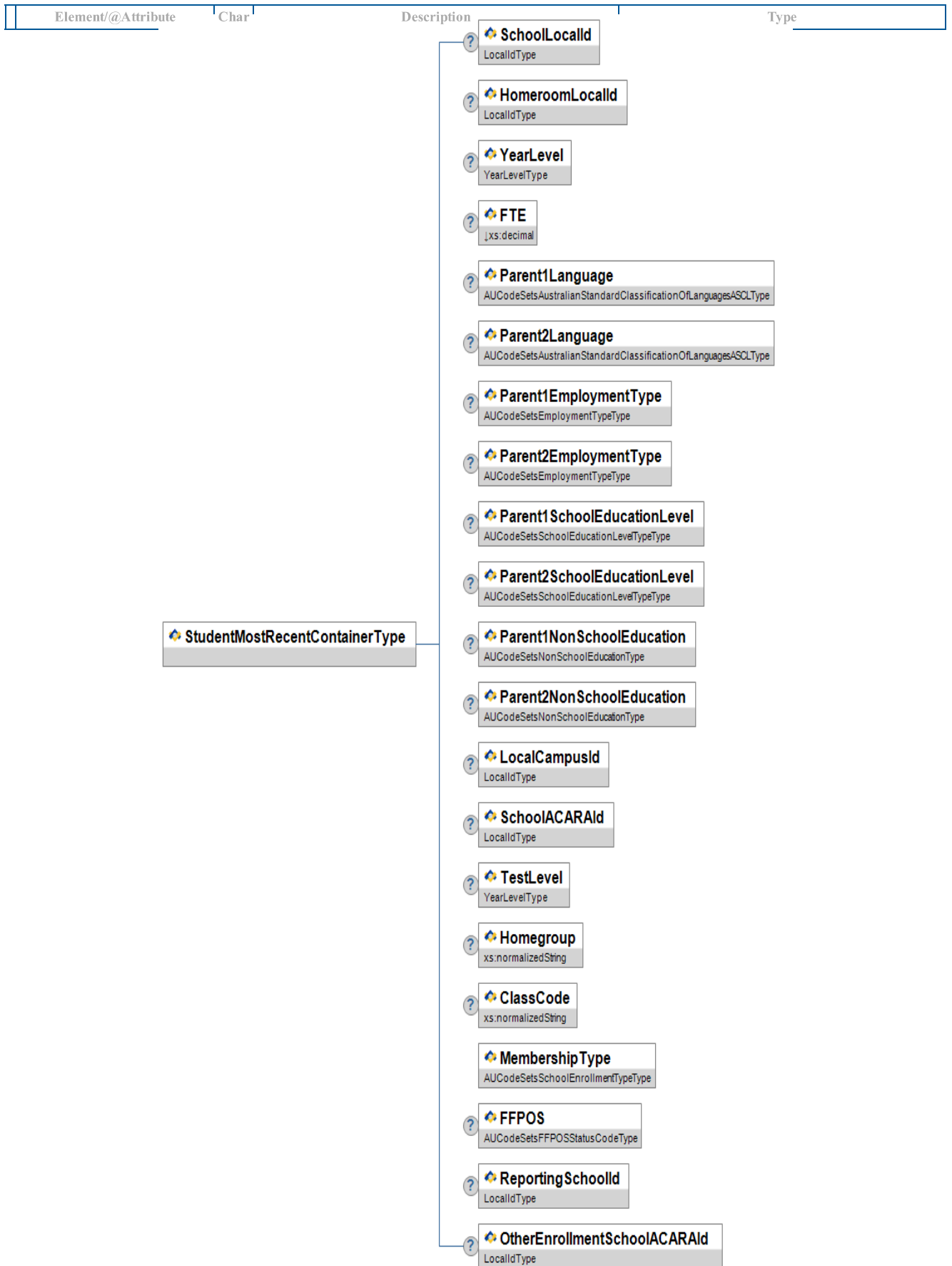
Figure A.169-1: StudentMostRecentContainerType
