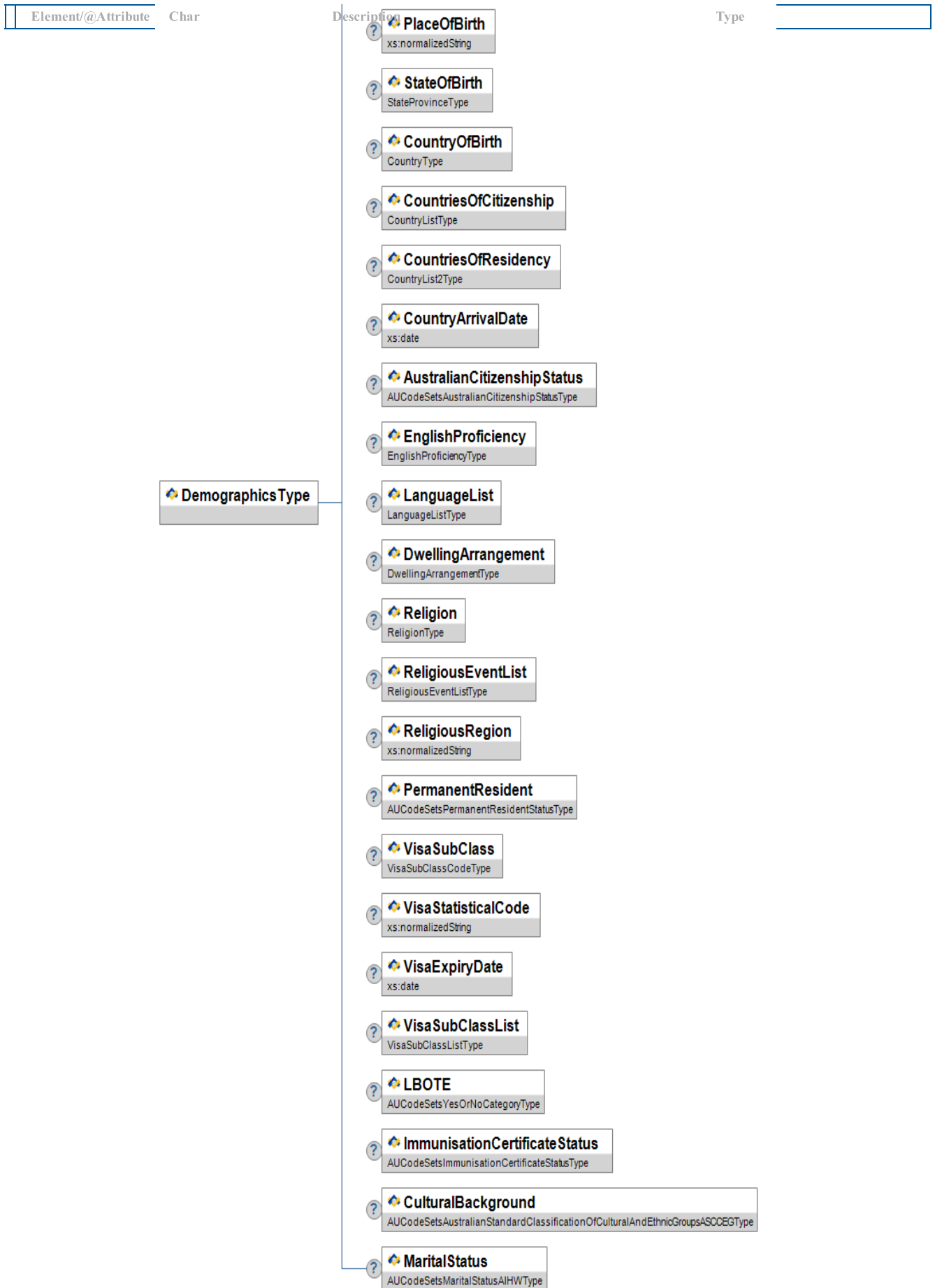
Figure A.44-1: DemographicsType
