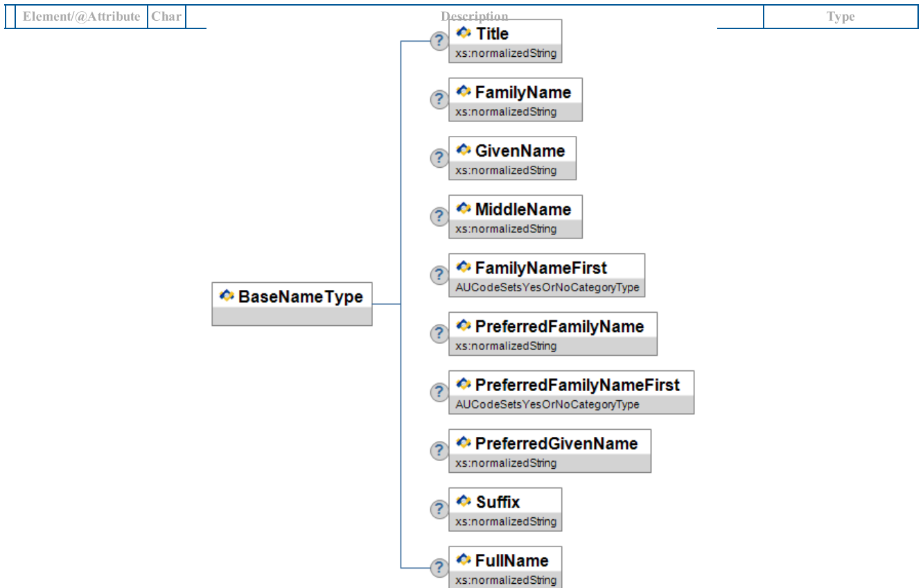
Figure A.24-1: BaseNameType
