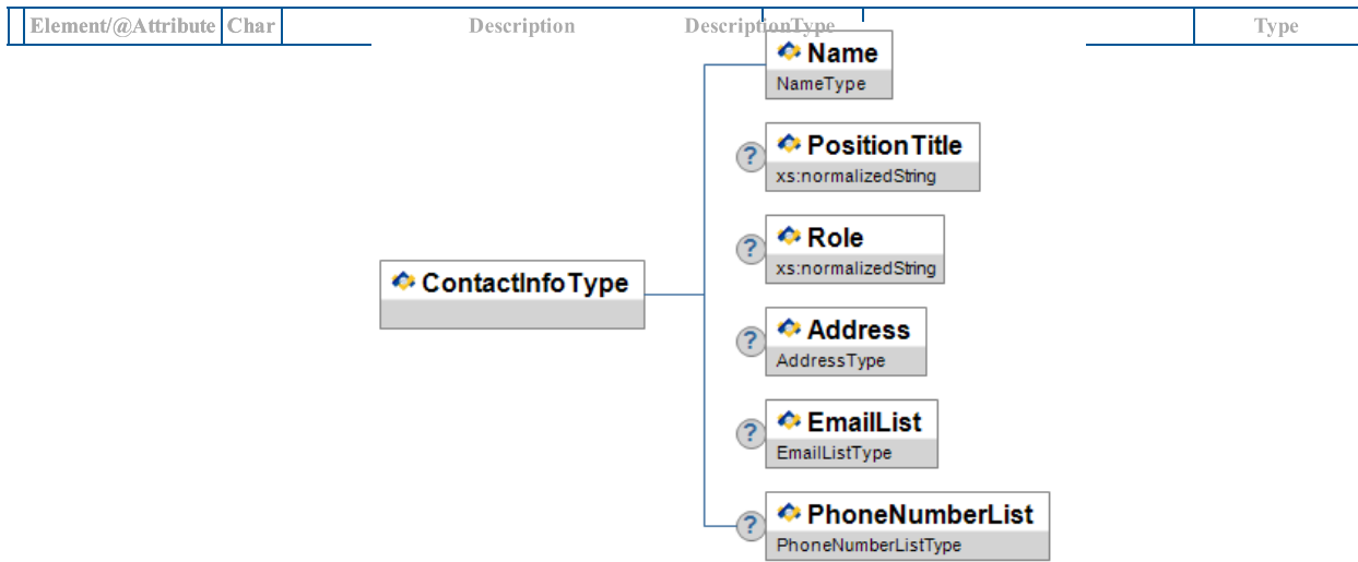
Figure A.34-1: ContactInfoType
