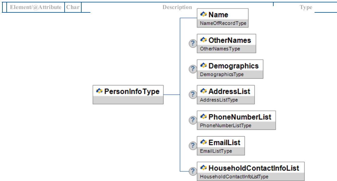
Figure A.107-1: PersonInfoType
