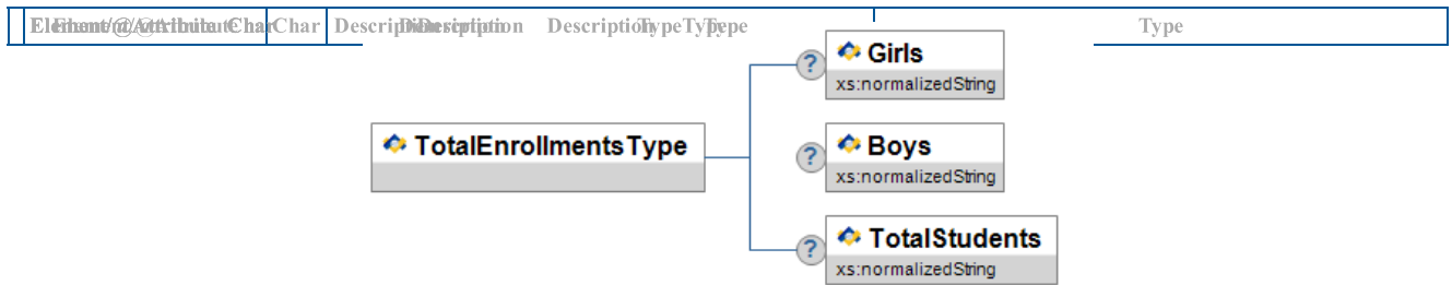
Figure A.190-1: TotalEnrollmentsType
