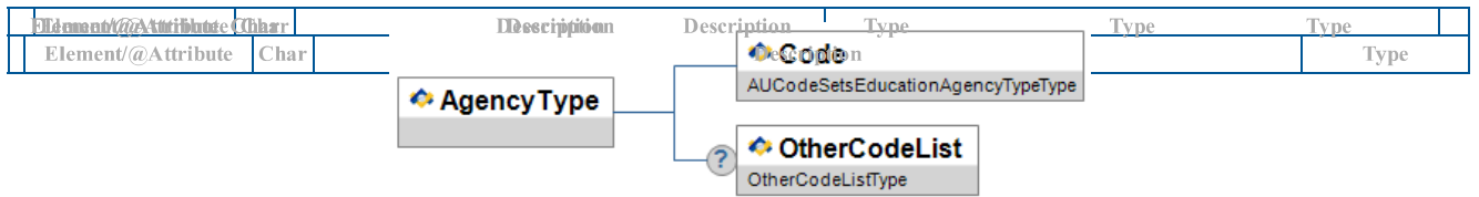
Figure A.11-1: AgencyType
