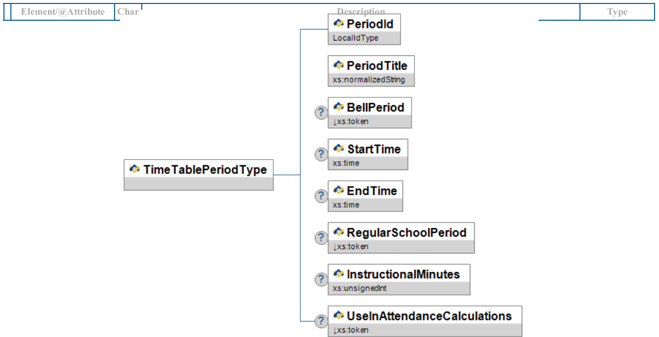
Figure A.189-1: TimeTablePeriodType
